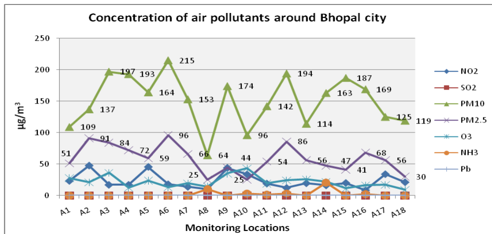
Figure 1: Concentration of air pollutants of Bhopal city
