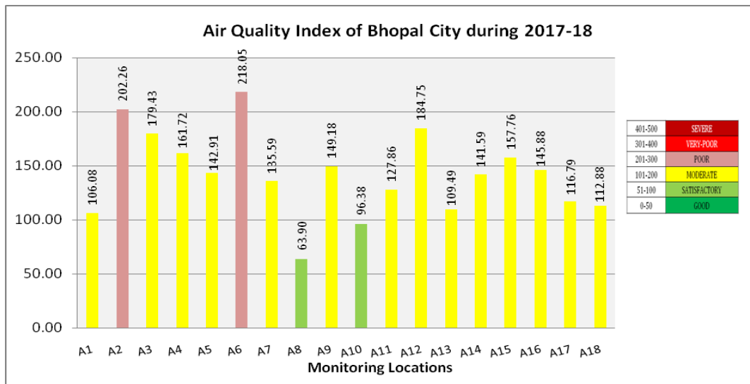
Figure 2: Air Quality Index of Bhopal City during year 2017-18
