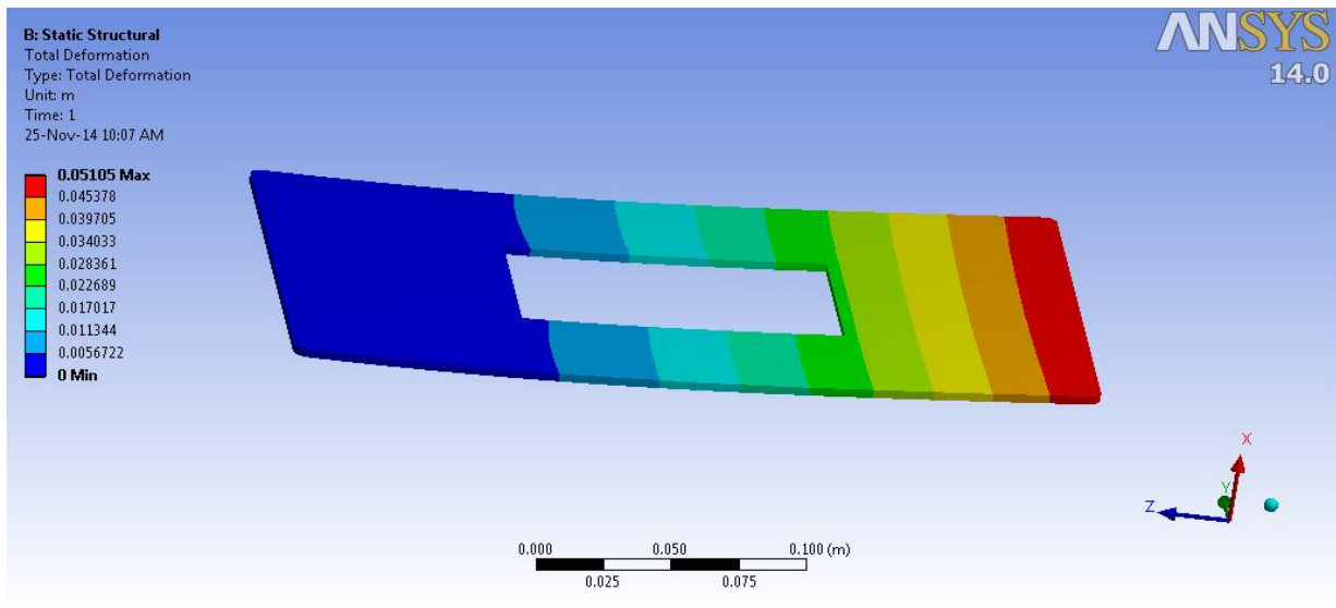
Fig 5.7 Rectangle Plate with Rectangle Cut-Out
