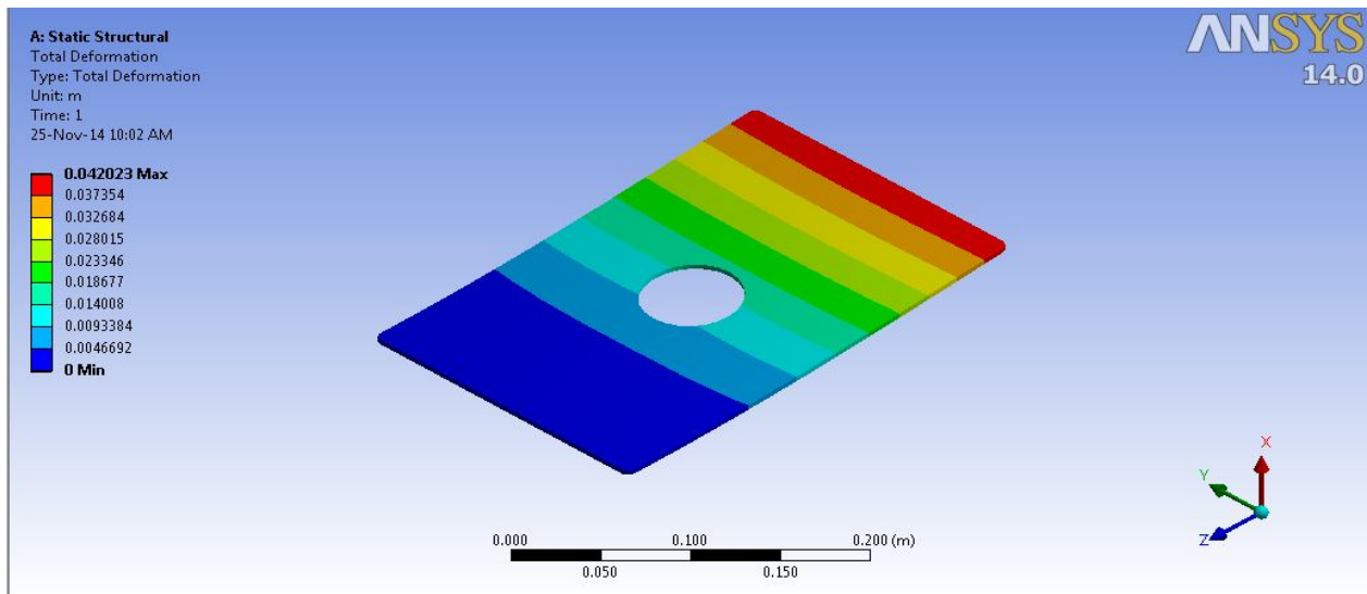
Fig 5.3 Rectangle Plate with Circular Cut-Out
