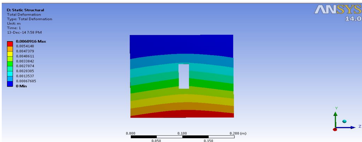
Fig 6.8 Square Plate with Rectangle Cut-Out
