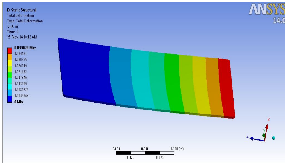
Fig 5.1 Rectangle Plate without Cut-Out
