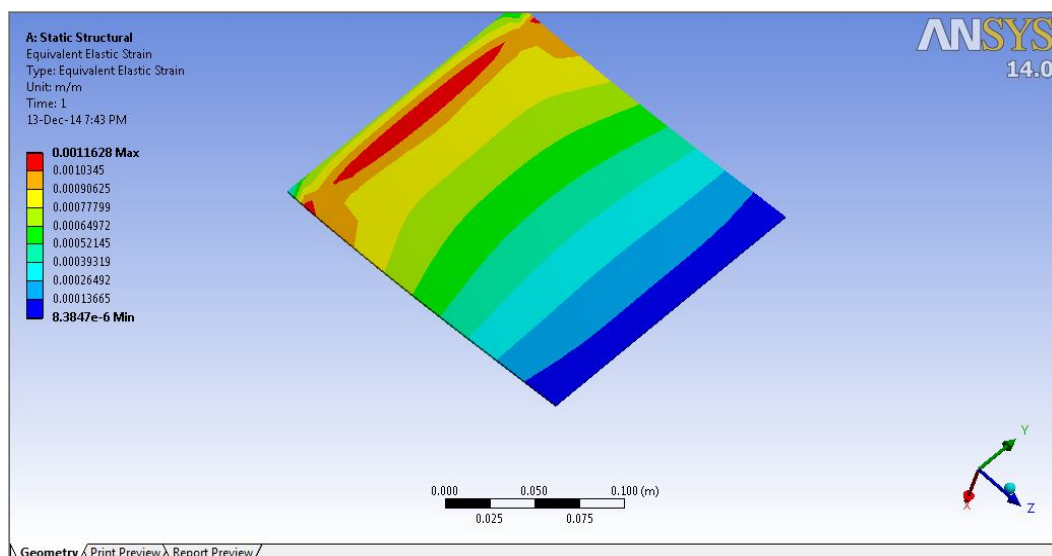
Fig 5.2 Square Plate without Cut-Out
