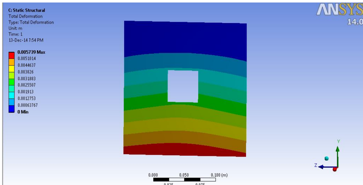
Fig 5.6 Square Plate with Square Cut-Out
