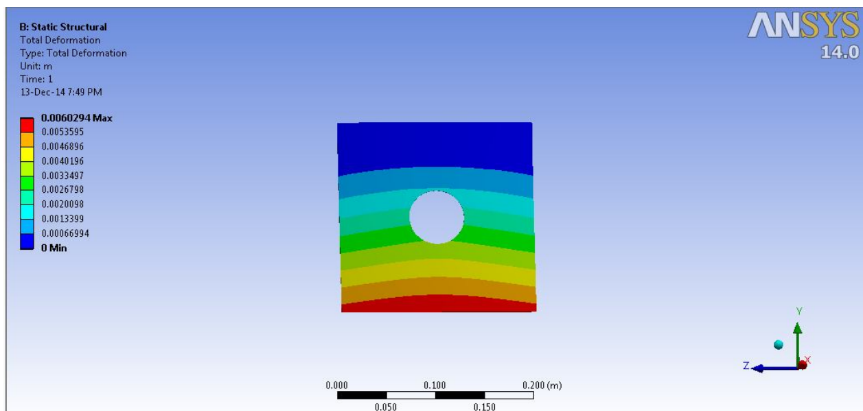
Fig 5.4 Square Plate with Circular Cut-Out
