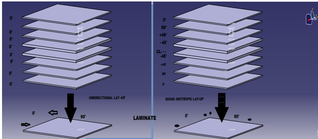
Fig 1.1 Laminate
