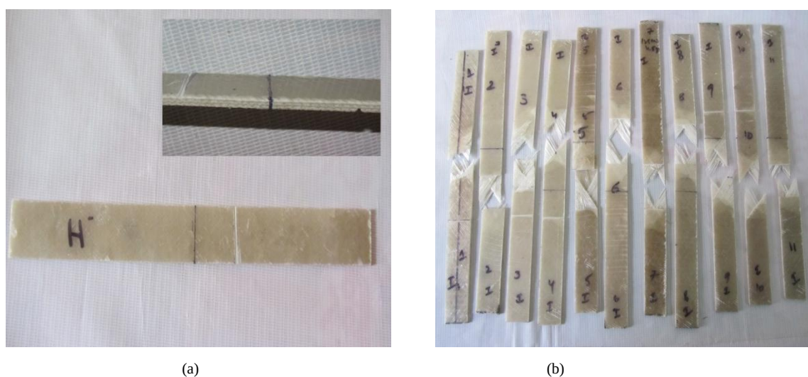
Fig 3.2: Sample for Inter laminar shear stress (b) samples after Inter laminar shear stress test
