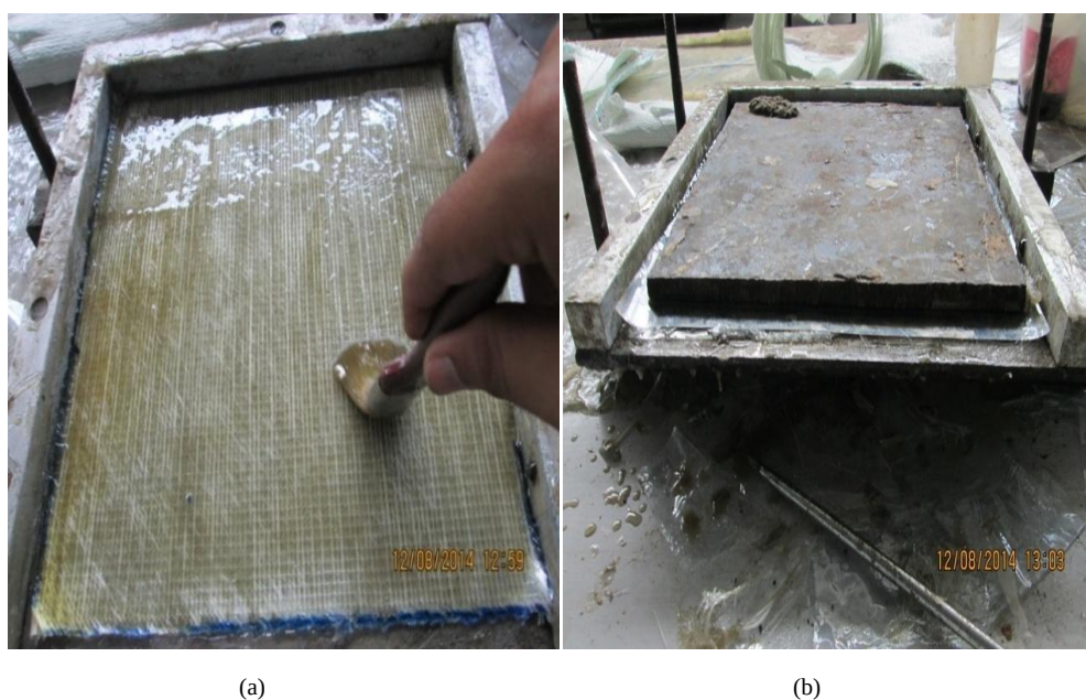
Fig. 2: (a) Hand layup of resin (b) placing the upper mold
