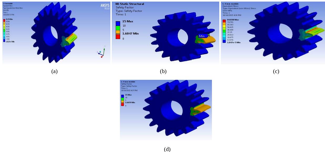
Fig. 4 (a) Von Mises Stress distribution in PEK spur Gear (b) Factor of Safety of PEK (c) Von Mises Stress distribution in Cast Iron spur Gear (d) Factor of Safety of Cast Iron
