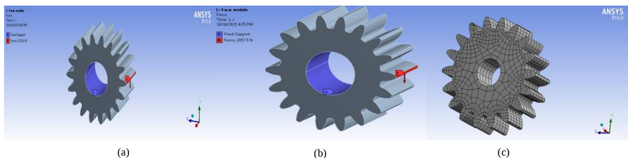
Fig. 3. (a) Boundary condition of PEK (b) Different fixed support and forces (c) Meshing of PEK Spur Gear
