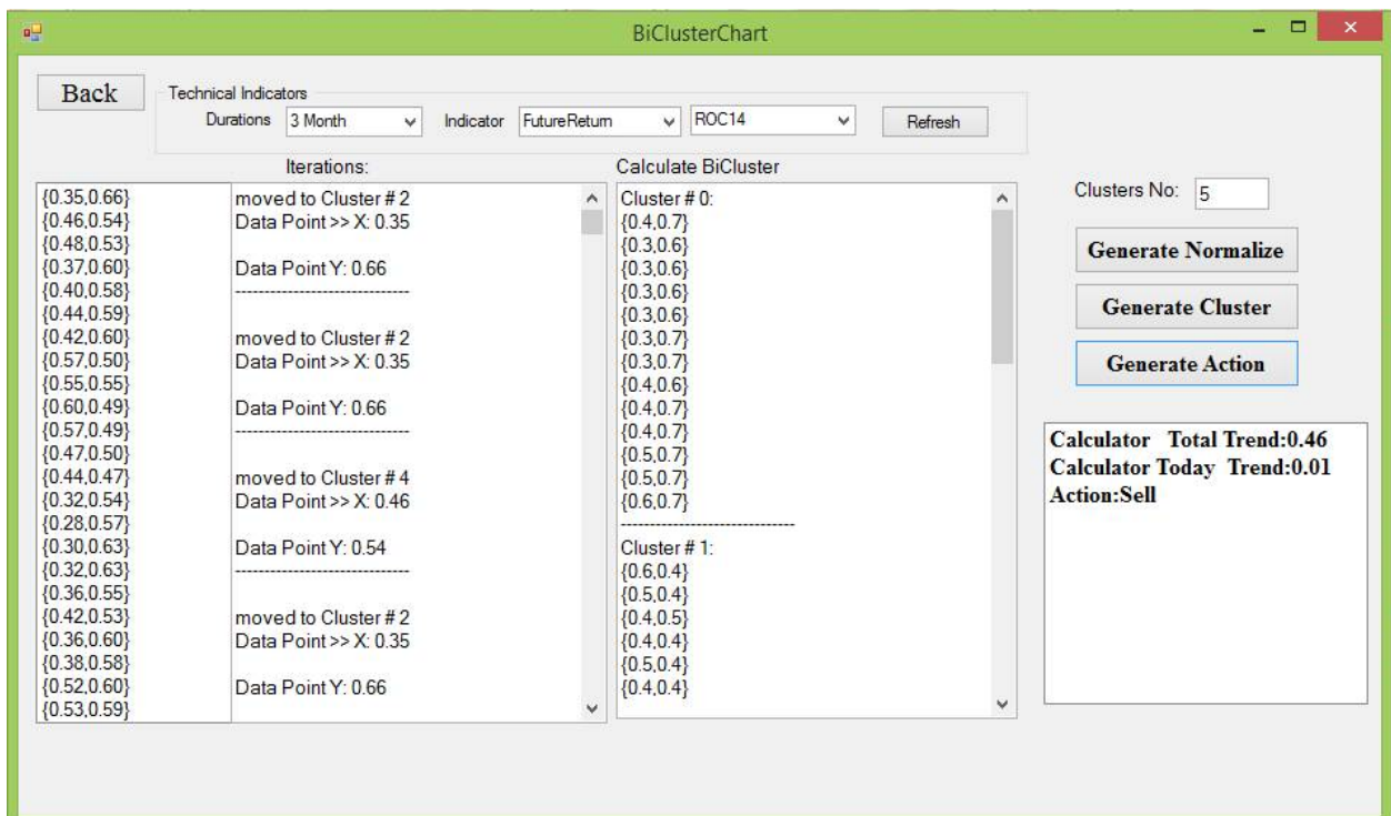
Figure 5: Trading Recommendation by system
