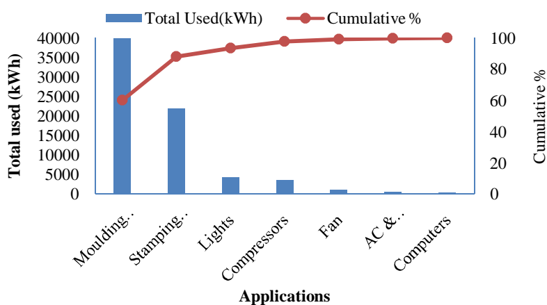
Figure (7): Application vs. Total kWh used(Pareto Chart)
