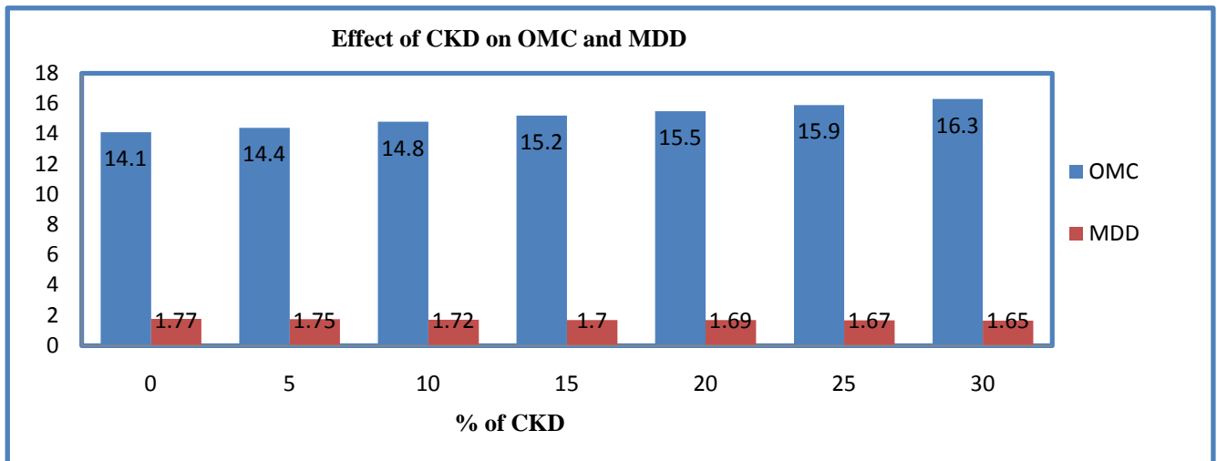
Fig. 1: OMC and MDD at varying percentages of CKD
