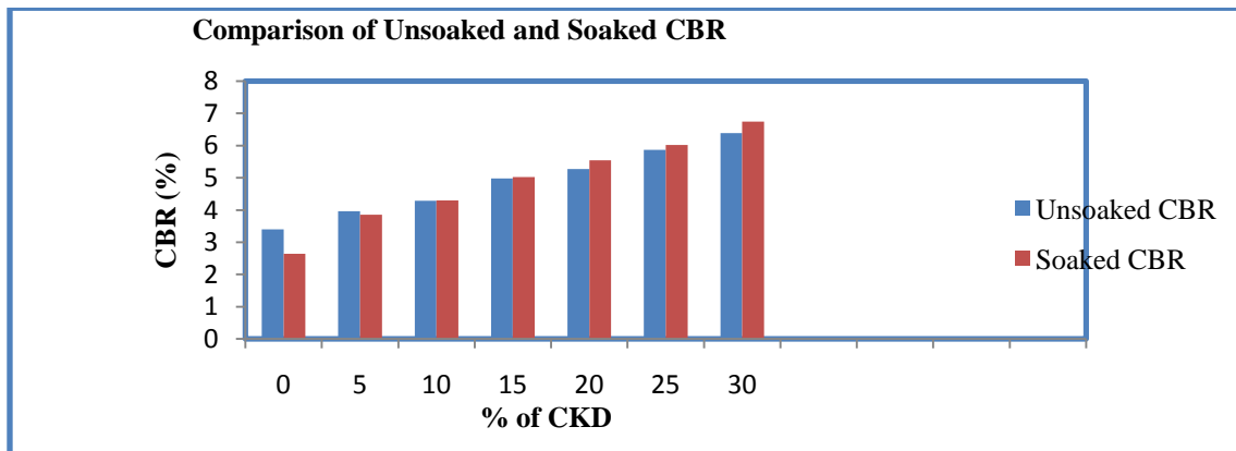
Fig.4: Unsoaked & Soaked CBR Variation of Soil-CKD Mix.
