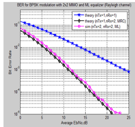
Figure.3 BER of 2*2 Alamouti STBC ML equalizer
