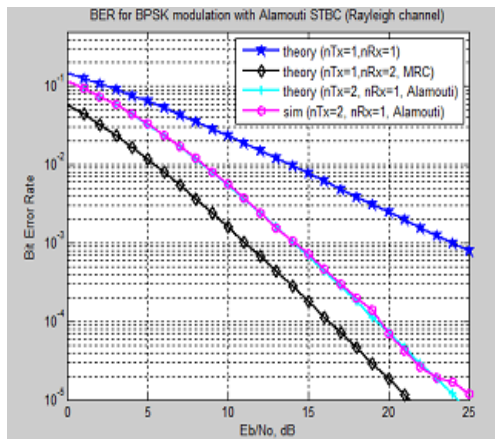
Figure.2 BER of 2*1 Alamouti STBC ML equalizer
