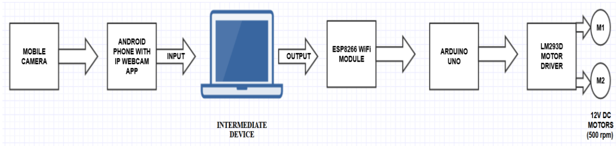
Fig 1: Block diagram of Robotic car controlled using Wi-Fi Module ESP8266
