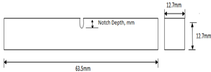
Fig 4.1 The dimensional view of specimen
