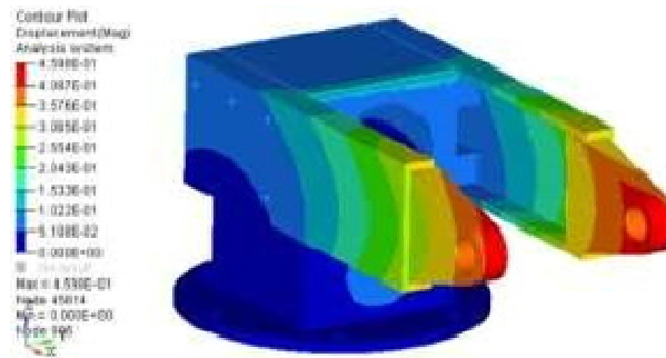
Fig. 7 Displacement Plot
