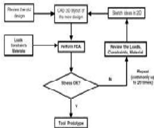
Fig. 2 Old Method to Solve Engineering Problem
