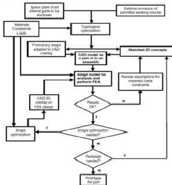
Fig. 3 New Method to Solve Engineering Problem
