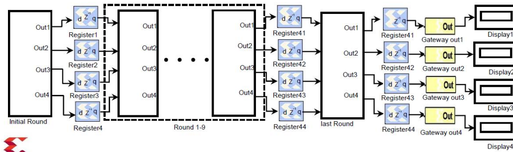
Figure 2: Architecture of our AES in System Generator
