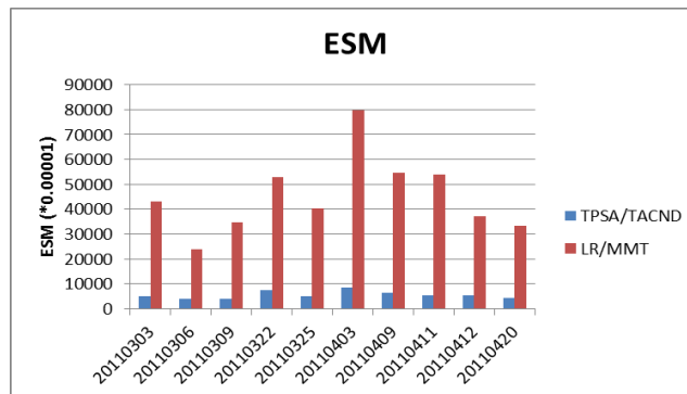
Figure5. Energy-SLAV-Migration
