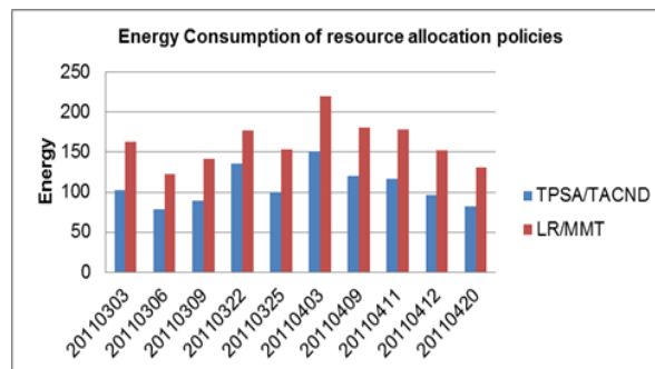
Figure 2. Energy Consumptions
