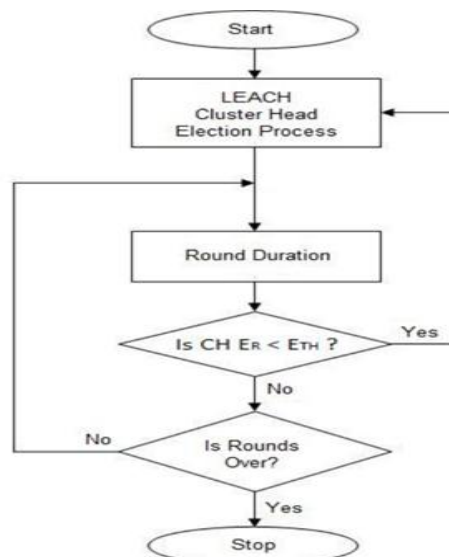
Figure 3: Dynamic Cluster Head Election Algorithm
