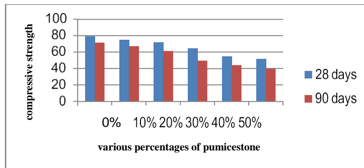
Fig. 9. Durability test in presence of HCL solution
