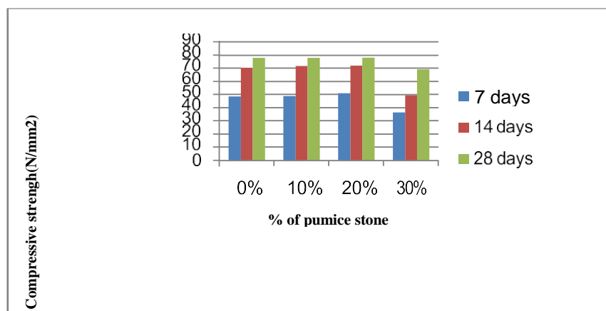
Fig. 4. Graph Showing Various Percentages of Pumice Stone
