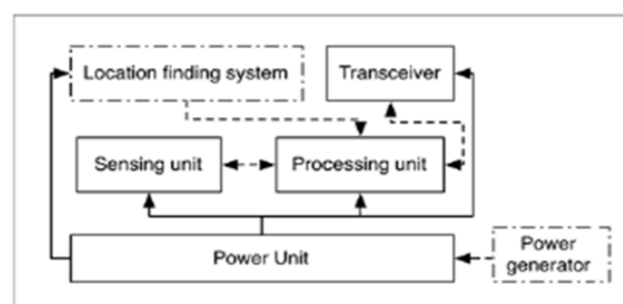
Figure 1: Functional blocks in a Sensor Node
