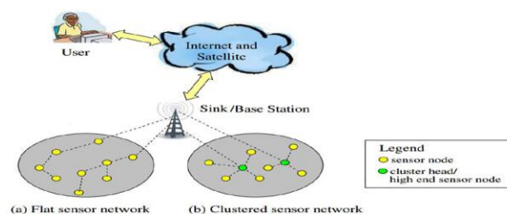
Figure 2: Architecture and operation of WSN
