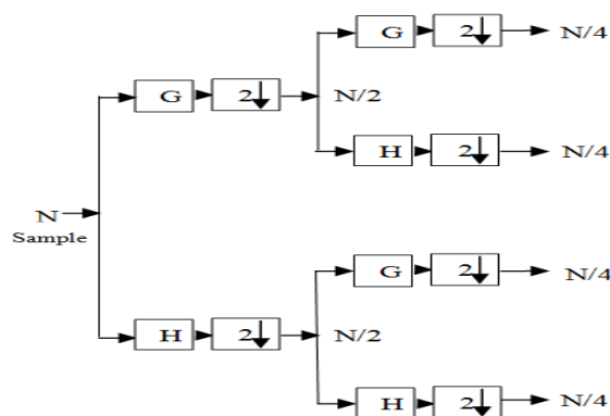
FIGURE 2: 2- LEVELS FOR DWT. WHERE G, H ARE THE HIGH-PASS AND LOW-PASS FILTER COEFFICIENT
