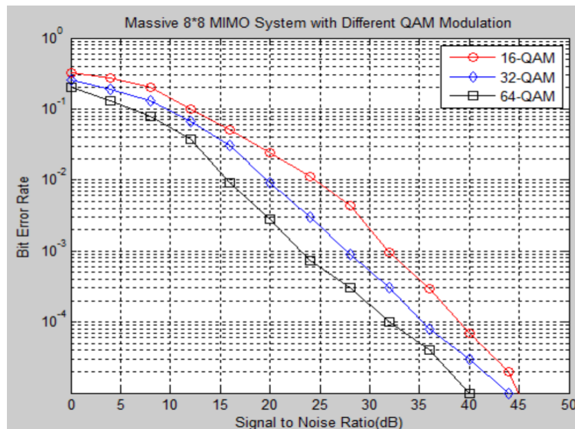
Figure 3: BER vs SNR for Massive 8 \times 8 System with QR-RLS based Channel Estimation Technique
