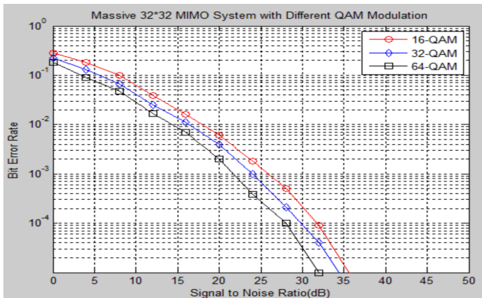
Figure 5: BER vs SNR for Massive 32×32 System with QR-RLS based Channel Estimation Technique
