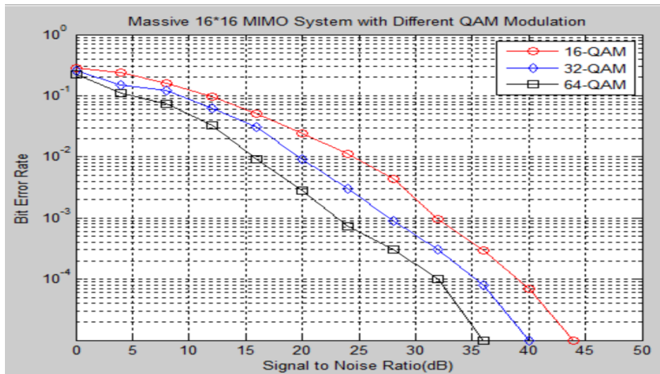
Figure 4: BER vs SNR for Massive 16×16 System with QR-RLS based Channel Estimation Technique
