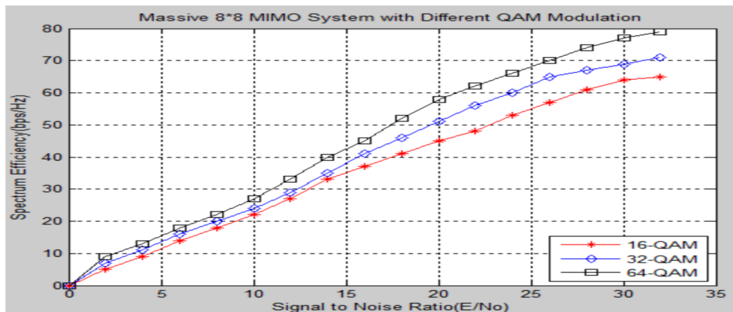
Figure 6: Spectrum Efficiency vs SNR for Massive 8x8 System with QR-RLS based Channel Estimation Technique
