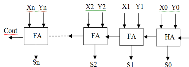
Figure 3: Parallel Adder (n=7 for SPFP and n=10 for DFPF)
