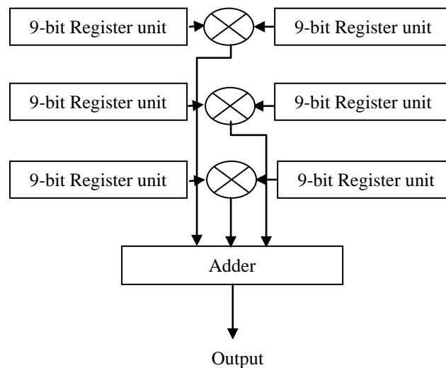
Figure 7: Proposed PPI – SO Design for n = 3
