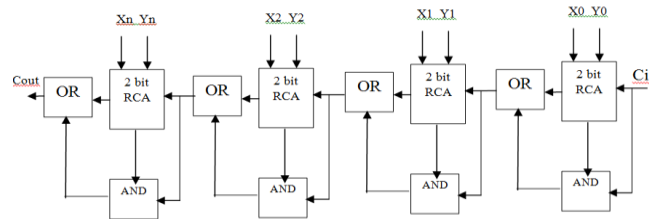
Figure 5: Carry Skip Adder
