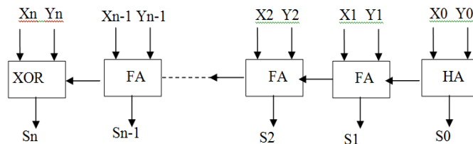
Figure 4: Modified Parallel Adder (n=7 for SPFP and n=10 for DPFP)
