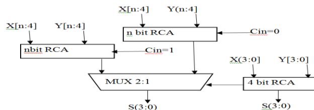
Figure 6: Carry Select Adder
