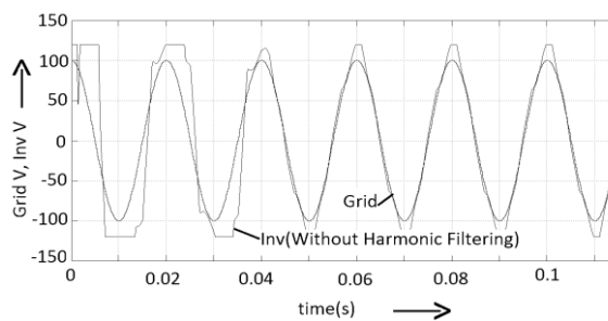
Fig. 8. Grid-V, Inv-V (Without using Filters)
