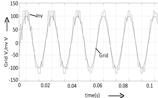
Fig. 9. Grid-V, Inv-V (with filters)
