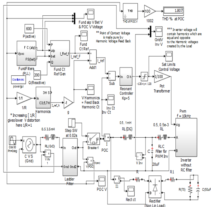
Fig. 2. Simulation block, Single Phase Inverter as DG
