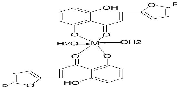
Figure-1: Metal complex of Manganese (II) with (E)-3-(furan-2-yl)-1-(2,6-dihydroxyphenyl)prop-2-en-1-one R = -H, M= Mn(II)
