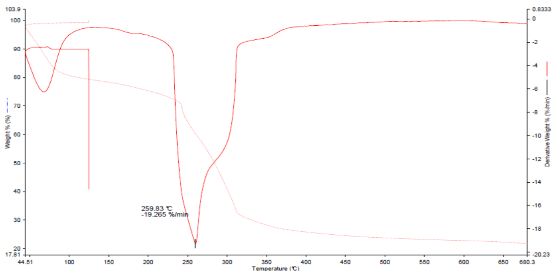
Figure-4: TG-DTA curve of Mn (II) complex of (E)-3-(furan-2-yl)-1-(2,6-dihydroxyphenyl)prop-2-en-1-one
