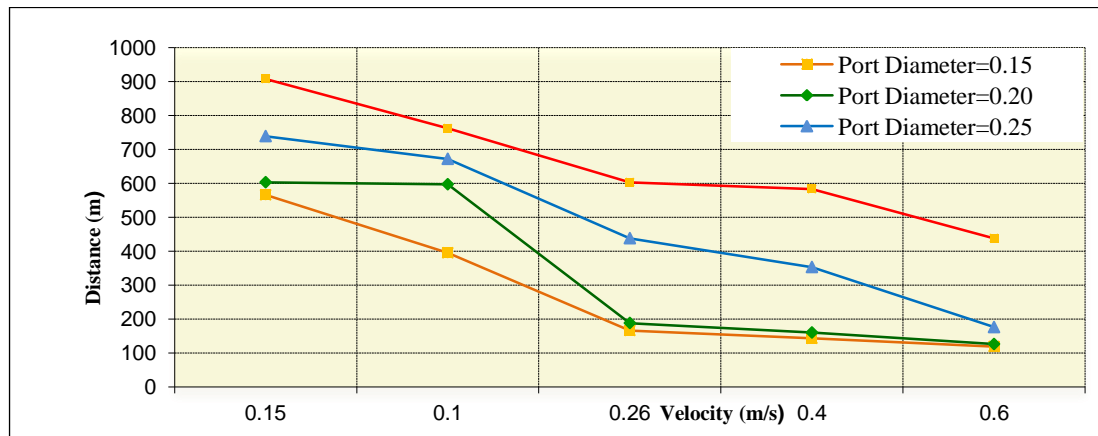
Figure 4: Dispersion Distance from Outfall for 0.1 ppt Concentration
