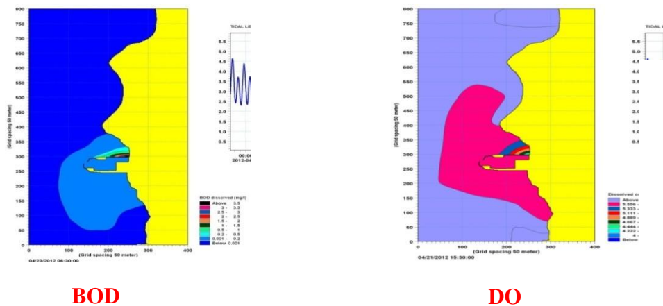
Figure 2: BOD and DO Distribution in the Nandgaon Region
