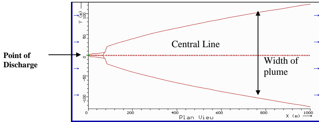
Figure3. : Salinity Distribution at Ennore Coastal area
