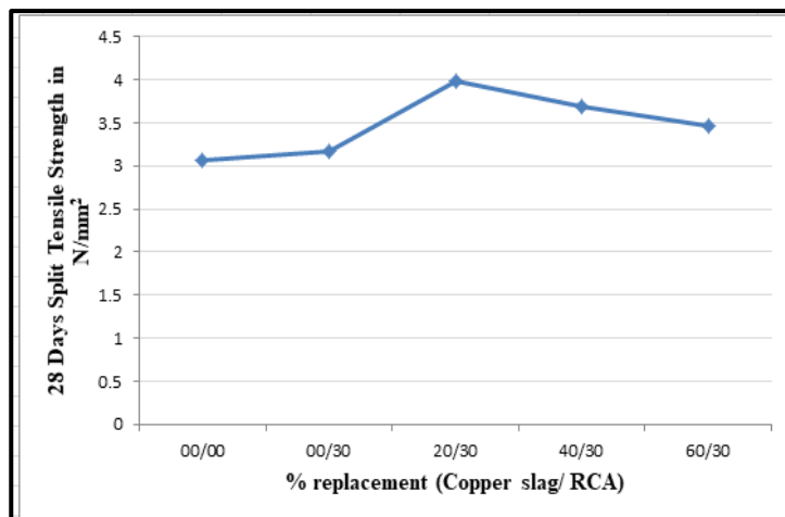
Fig 8: Variation in split tensile strength
