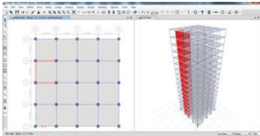
Fig 2 Model 2 - Square Geometry
