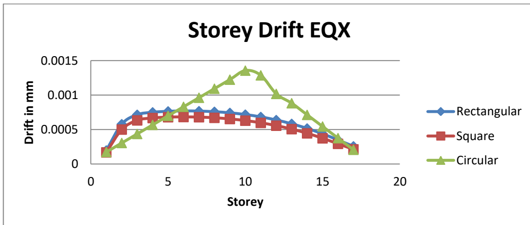
Graph 3: Storey Drift EQX
