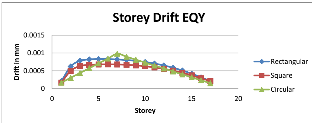
Graph 4 : Storey Drift EQY
