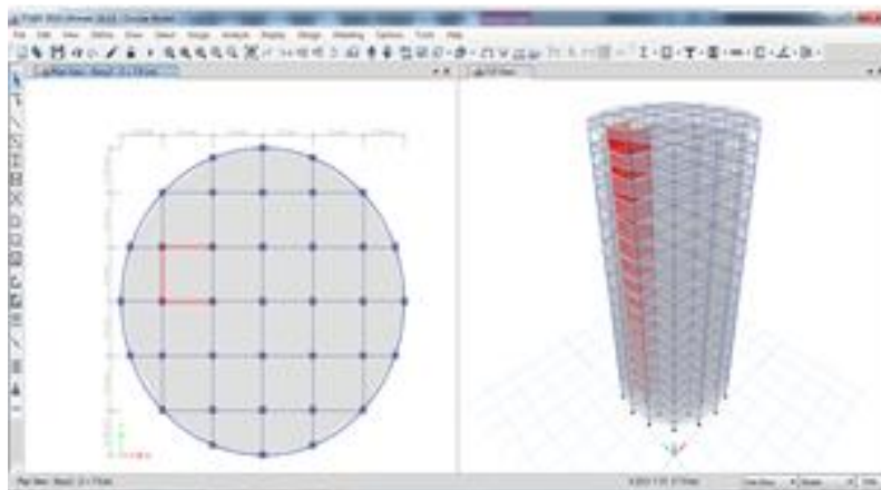
Fig 3 Model 3 - Circular Geometry
