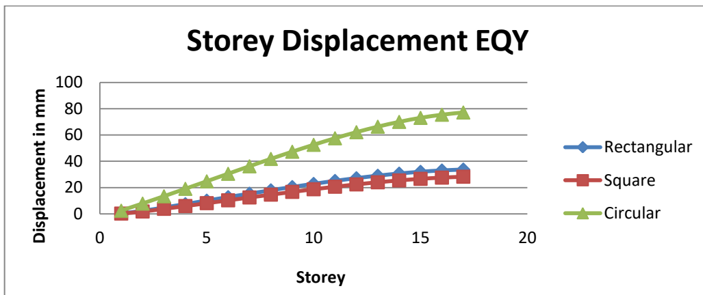
Graph2 : Storey Displacements EQY
