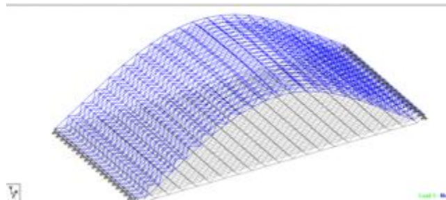
Fig 5 Mode Shape 3 for Flat Roof
