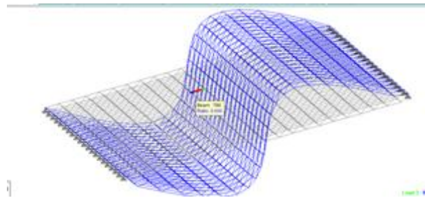
Fig 4 Mode Shape 2 for Flat Roof
