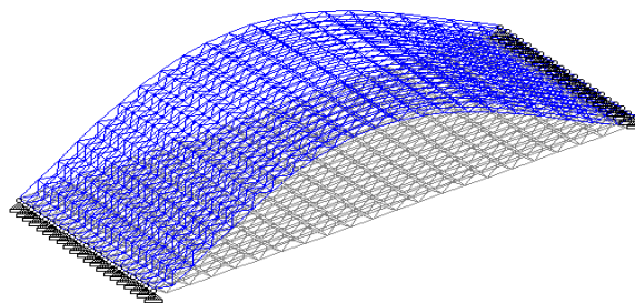
Fig 11 Mode Shape3 for Inclined Roof
