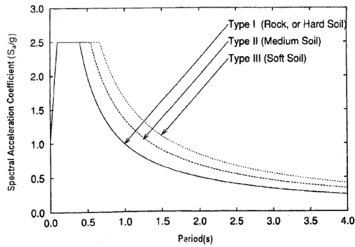
Fig 2 IS Code Spectra From IS 1893:2002 (Part I)
