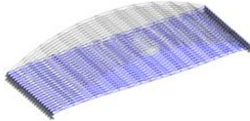
Fig 6 Mode Shape 1 for Curved Roof
