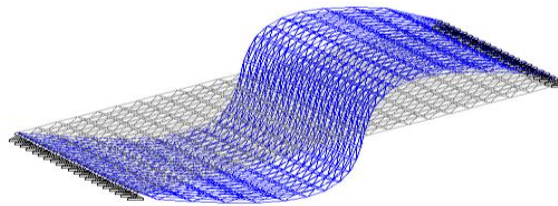
Fig 10 Mode Shape2 for Inclined Roof
