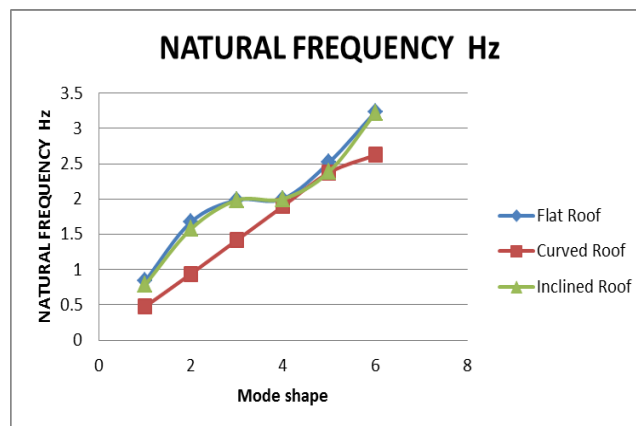
Fig 12 Graphical Representation of Flat Curved and Inclined Roof for Natural Frequency Vs. Mode No
