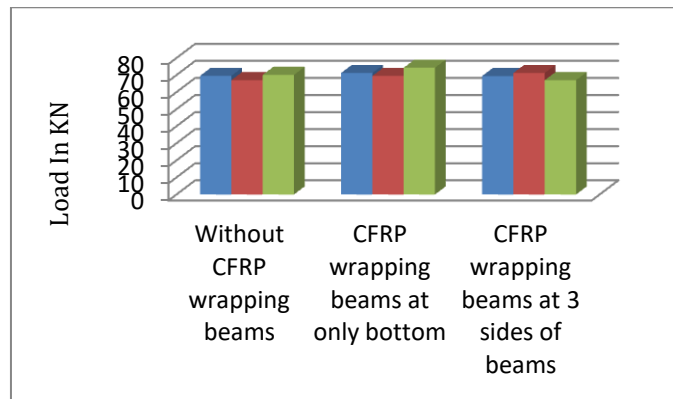
Fig. 3. Load Carrying by Fly ash and GGBS using RC beams
