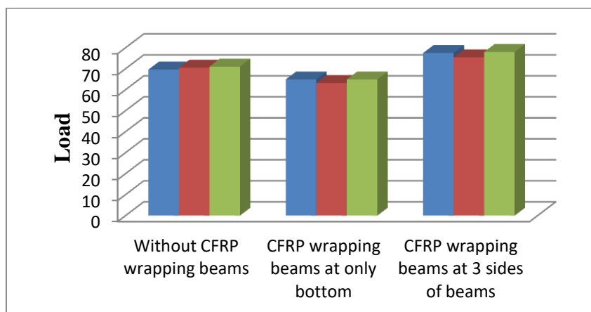
Fig. 5. Load Carrying by Fly ash used RC beams
