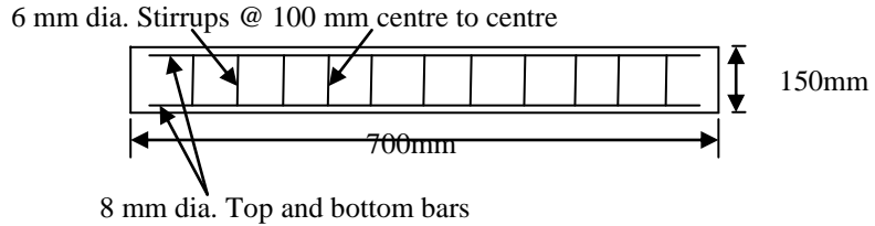
Fig. 1. Longitudinal section of beam
