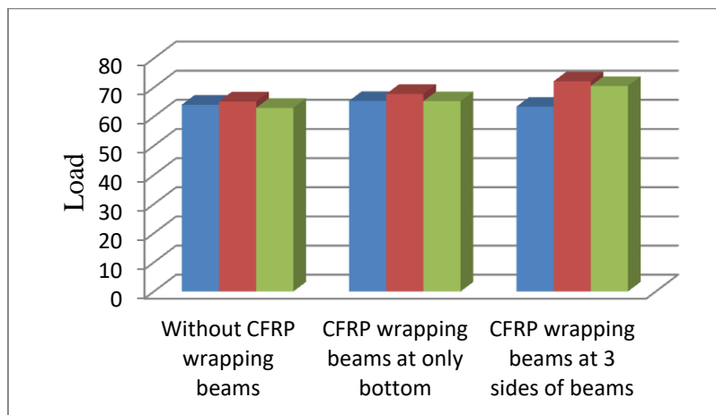
Fig. 6. Load Carrying by Fly ash used RC beams (Cement replaced with 30% fly ash)
