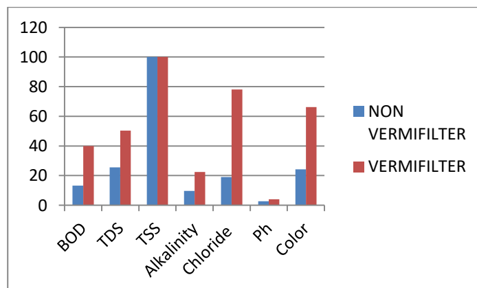
Fig.7. Graph showing comparison of filters at hydraulic loading rate of 40 l/m 2 /day
