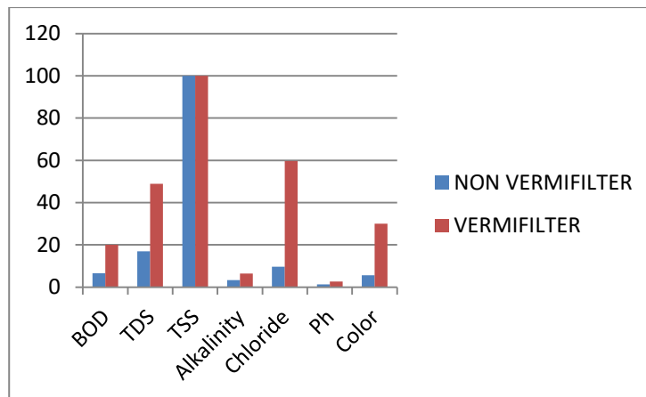
Fig.8. Graph showing comparison of filters at hydraulic loading rate of 55 l/m 2 /day
