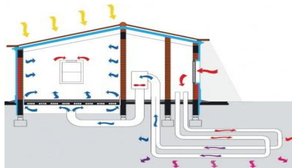
Fig 2: Open type earth tube heat exchanger [8]
