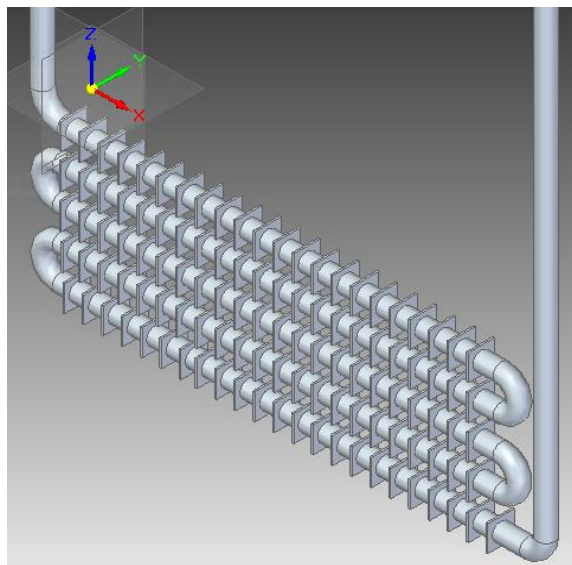
Fig 5: Fins at the ETHE
