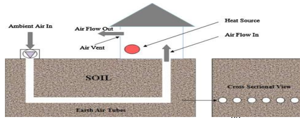
Fig -1: Earth tube heat exchanger [9]
