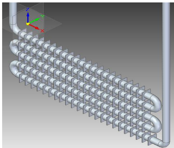
Fig 5: Fins at the ETHE
