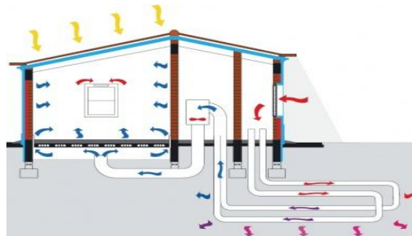
Fig 2: Open type earth tube heat exchanger [8]
