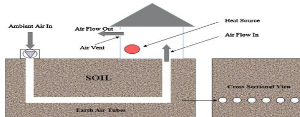
Fig -1: Earth tube heat exchanger [9]
