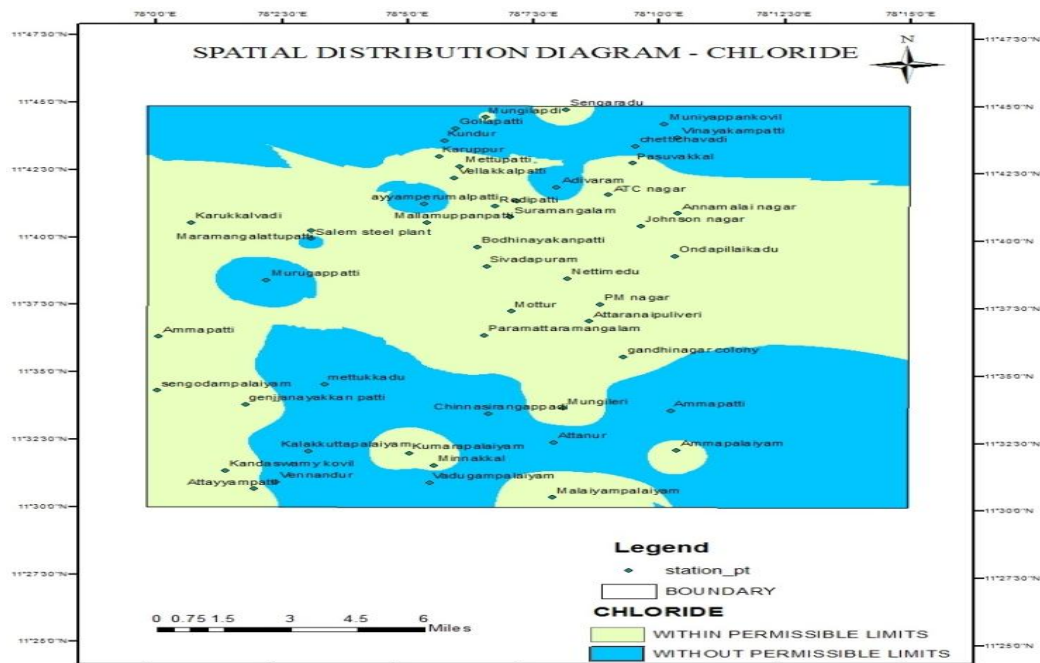
Figure 4: Spatial Distribution Diagram for Chloride in Study Area
