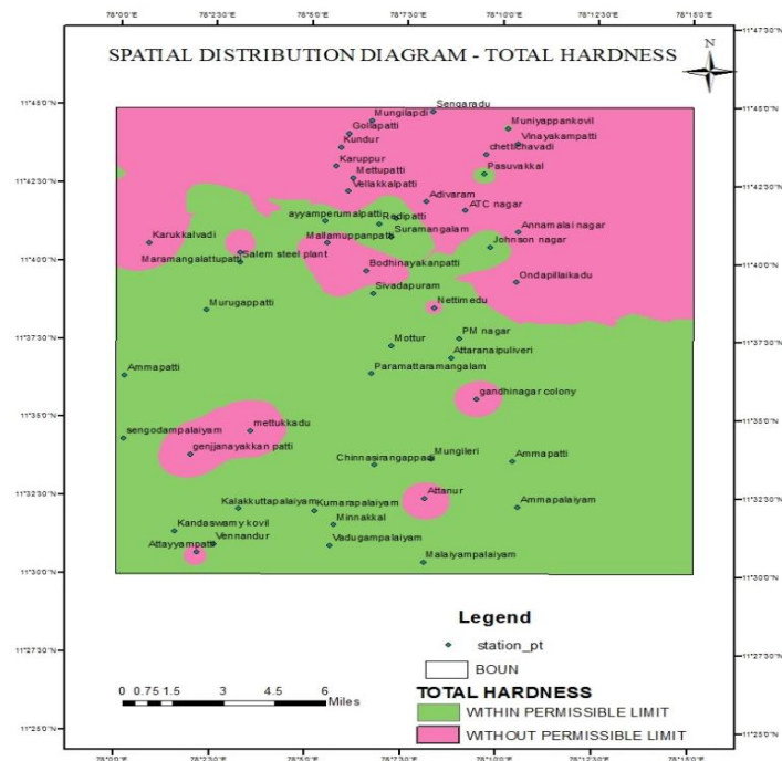
Figure 6: Spatial Distribution Diagram for Total Hardness in Study Area
