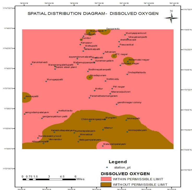
Figure 10: Spatial Distribution Diagram for Dissolved Oxygen in Study Area
