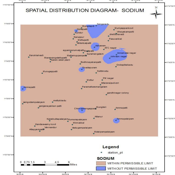
Figure 9: Spatial Distribution Diagram for Sodium in Study Area
