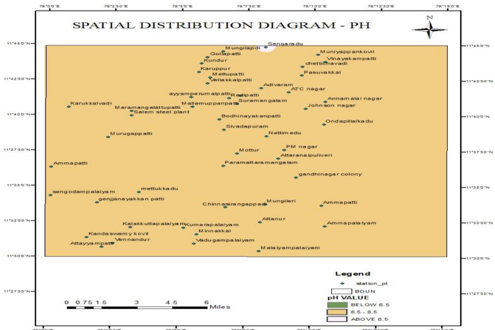
Figure 2: Spatial Distribution Diagram for pH in Study Area
