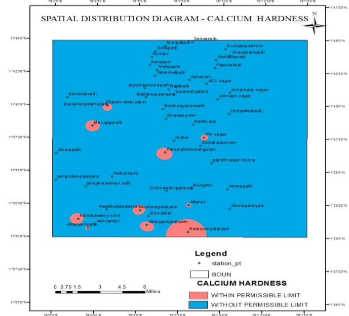
Figure 7: Spatial Distribution Diagram for Calcium Hardness in Study Area
