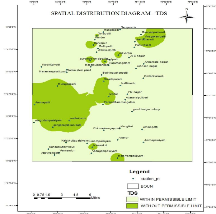
Figure 5: Spatial Distribution Diagram for Total Dissolved Solids in Study Area
