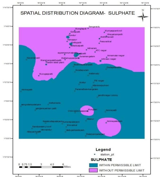
Figure 13: Spatial Distribution Diagram for Sulphate in Study Area.
