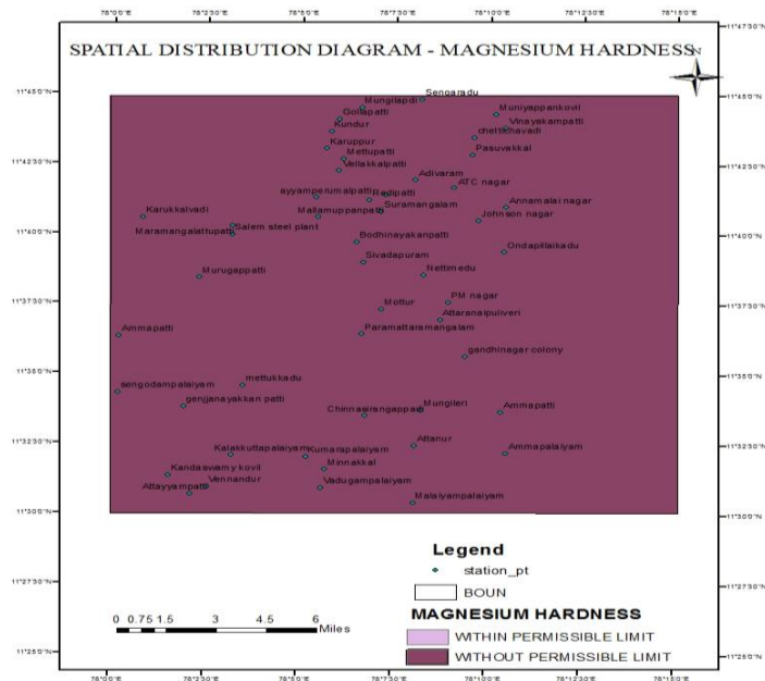
Figure 8: Spatial Distribution Diagram for Magnesium Hardness in Study Area
