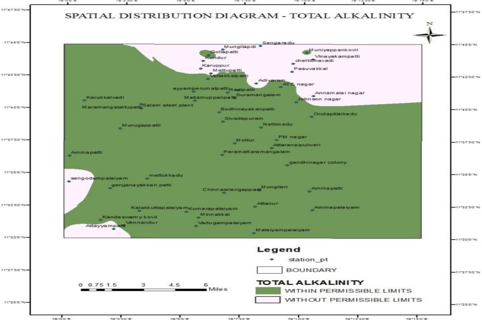
Figure 3: Spatial Distribution Diagram for Total Alkalinity in Study Area
