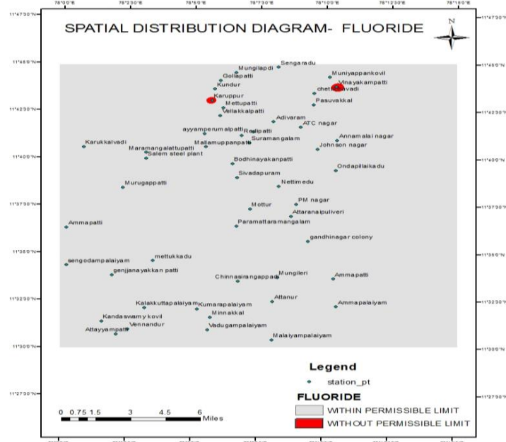
Figure 11: Spatial Distribution Diagram for Fluoride in Study Area
