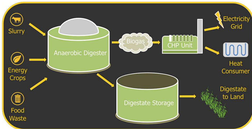
Figure 5: Anaerobic digestion
