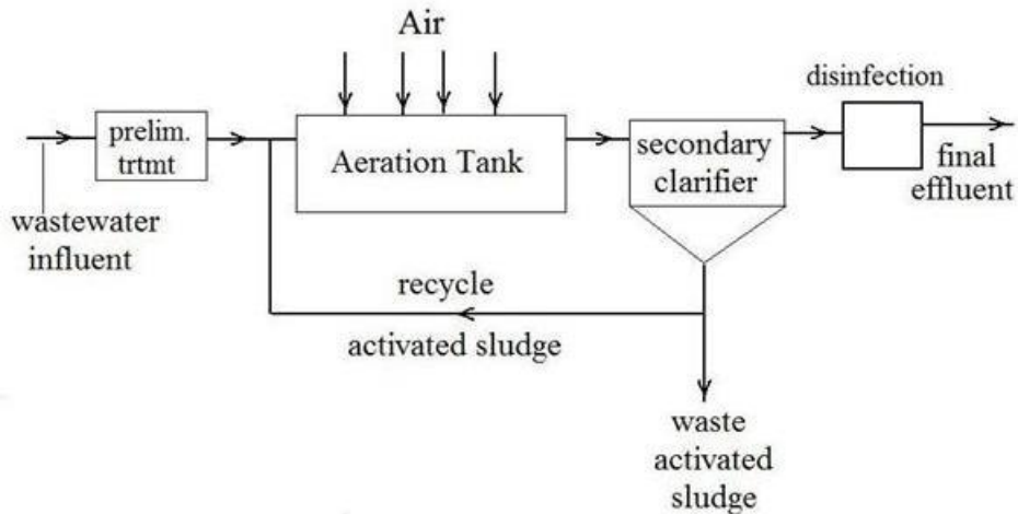
Figure 6: Activated Sludge Process (Flow diagram)
