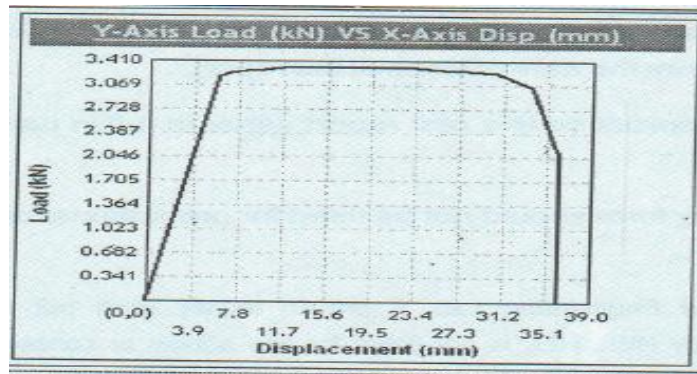
Fig.10. Results of Tensile test on Specimen A2.
