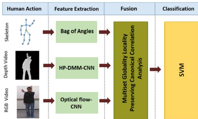
Figure 6: The proposed human action recognition framework using MGLPCCA [6]
