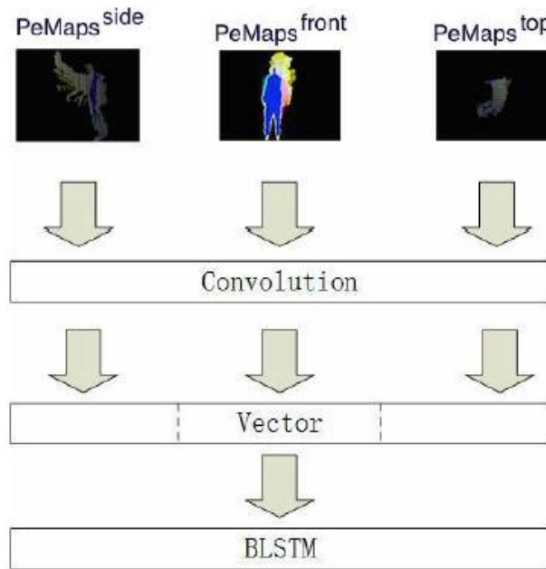
Fig. 5 Fusion method for PeMaps from different views [5]
