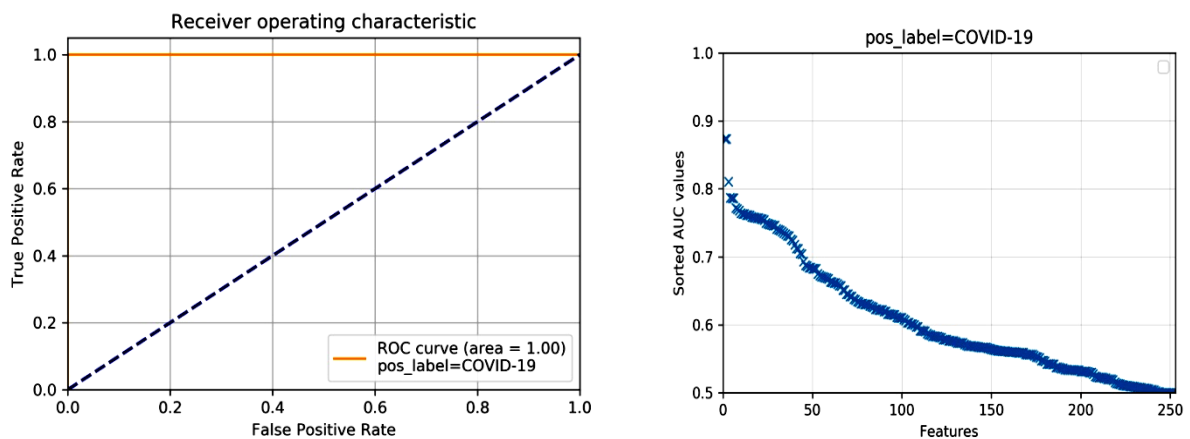
Figure 8: (a) ROC Curve (b) AUC curve
