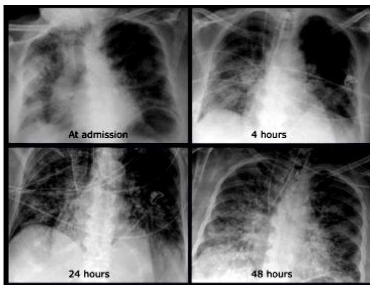
Figure 2: Chest condition due to Covid-19
