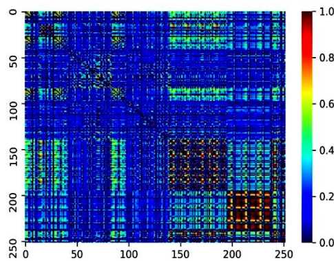
Figure 7: Correlation map
