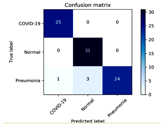
Figure 6: Confusion matrix
