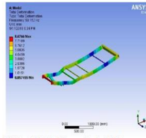
Fig. 7 Mode No.9 Natural Frequency (Bending Mode)
