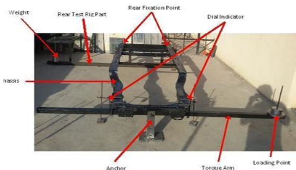
Fig.14 Actual model of torsional test rig.
