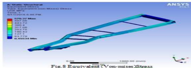
Fig.8 Equivalent (Von-mises) Stress
