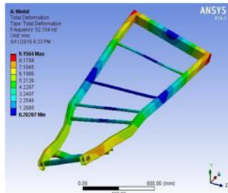
Fig.6 Mode No. 7 Natural Frequency (Torsional Mode)
