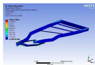
Fig.5 Equivalent (Von-mises) Stress
