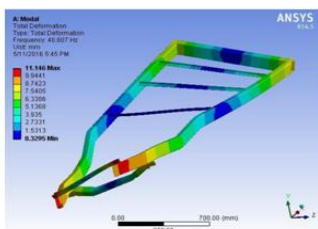
Fig.3 Mode No. 7 Natural Frequency (Torsional Mode)
