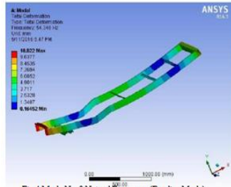
Fig.4 Mode No. 9 Natural Frequency (Bending Mode)
