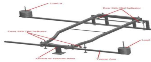
Fig.13 CAD model of torsional test rig.
