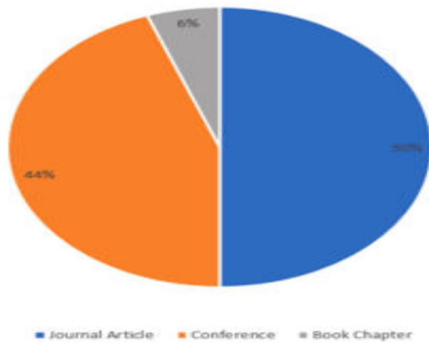
Figure 2: Type of Publications
