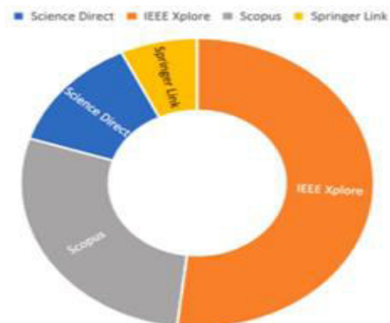
Figure 3: The distribution of studies per search database
