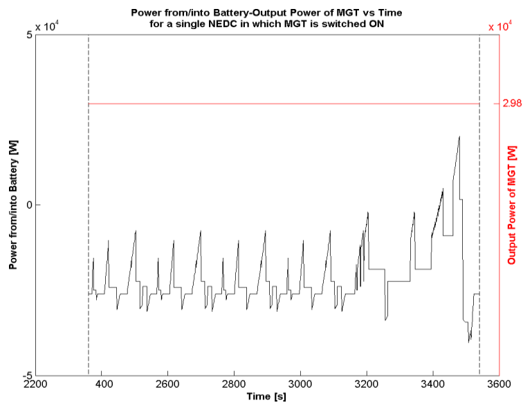
Figure 3: Power during a single NEDC in which the MGT is switched-on
