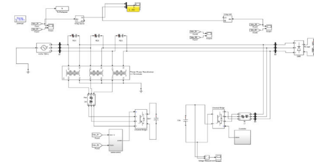
Fig.11 Simulink model with DPFC
