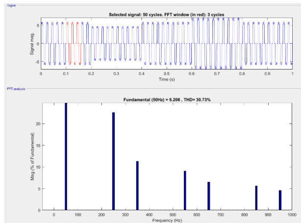
Fig.10 Representation of Total Harmonic Distortion without DPFC
