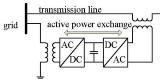
Fig. 1 Simplified representation of a UPFC
