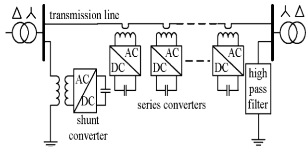
Fig. 3 DPFC Configuration
