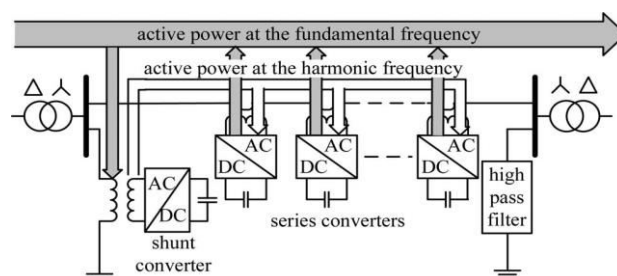
Fig. 4 Active power exchange between DPFC Converters
