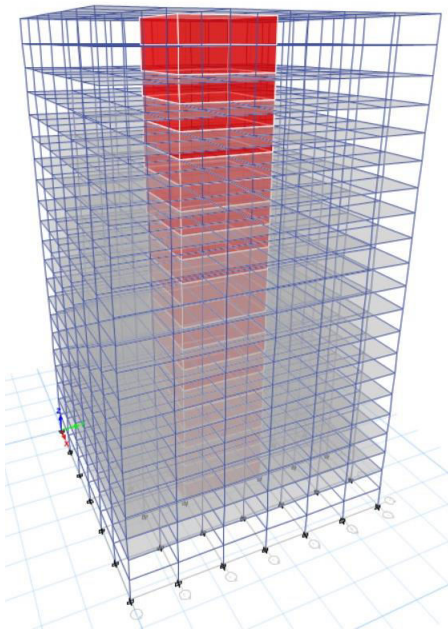
Model from ETABS of shear wall system
