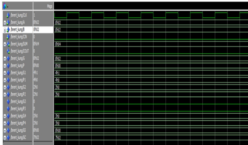
Figure 2. Brent Kung Waveform
