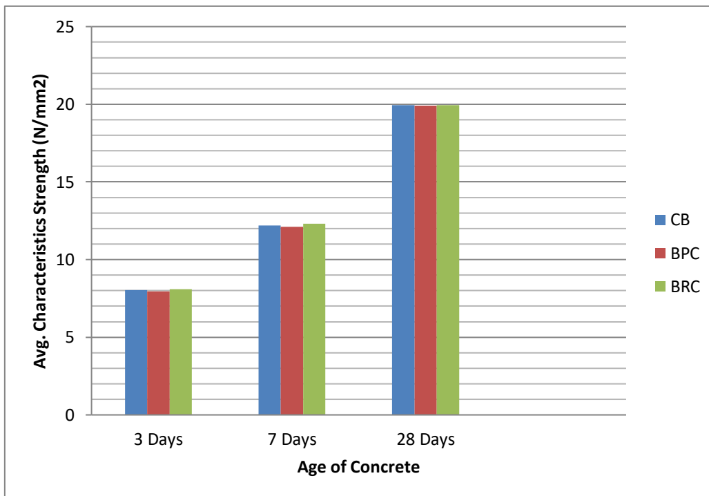
Fig 9.1 COMPARISION OF COMPRESSIVE STRENGTH OF CONCRETE
