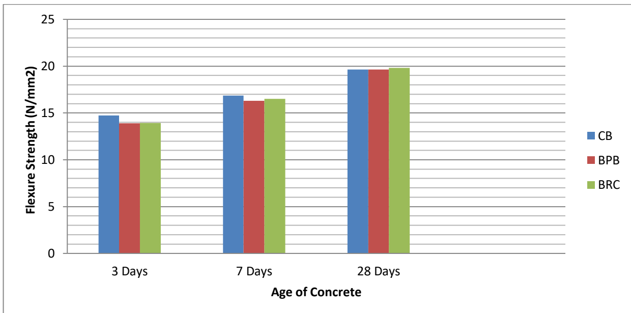
Fig.9.2 COMPARISION OF FLEXURE STRENGTH OF CONCRETE
