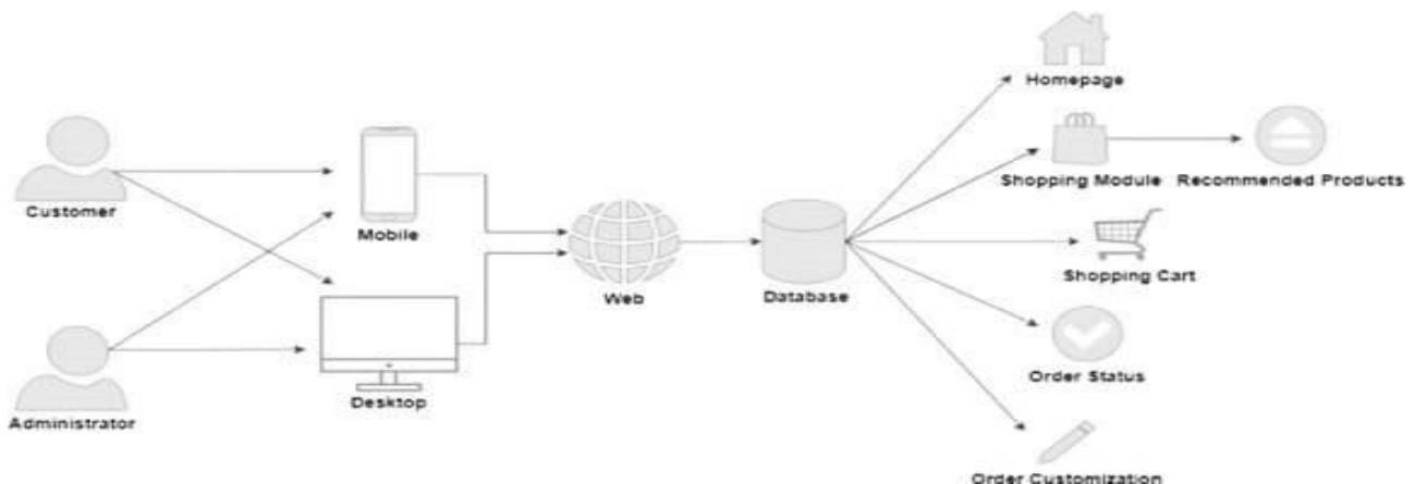
Figure 1: Methodology
