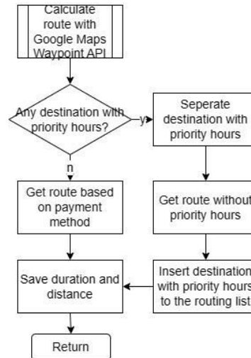
Fig 4. Routing algorithm
