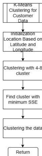
Fig 2. K-Means clustering algorithm
