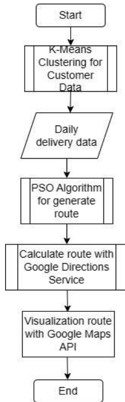
Fig 1. Main algorithm
