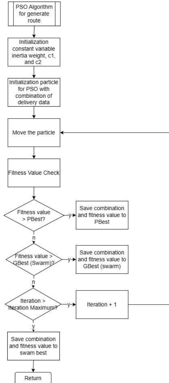
Fig 3. PSO algorithm
