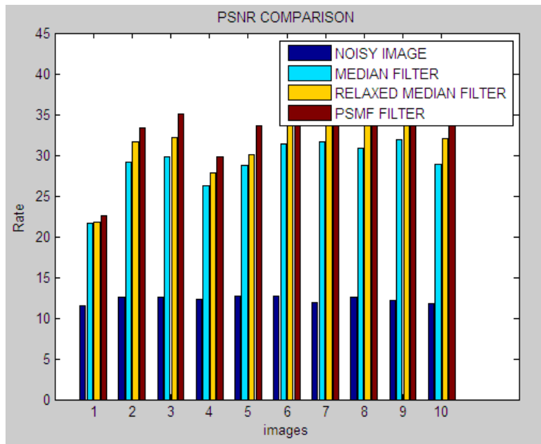
Fig 4.2:- PSNR evaluation
