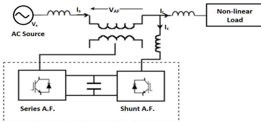
Figure 2. Basic Configuration of UPQC
