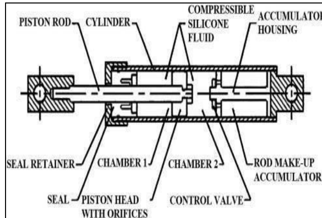
Figure 1: Cross Section of Fluid Viscous Damper
