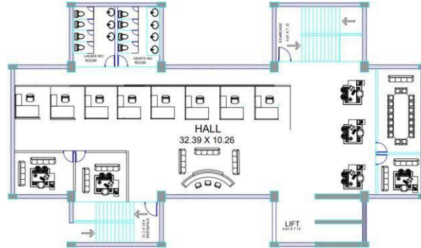
Figure 4: 1-15 Floor Plan
