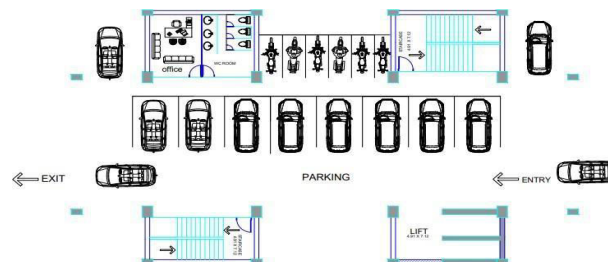
Figure 3: Ground Floor Plan
