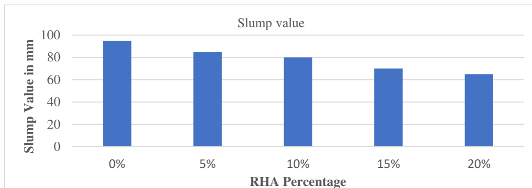
Figure 2: Workability of concrete with RHA
