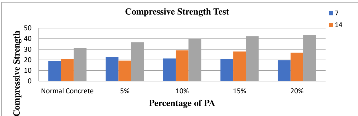
Figure 5: Compressive strength of concrete for varying percentage of PA
