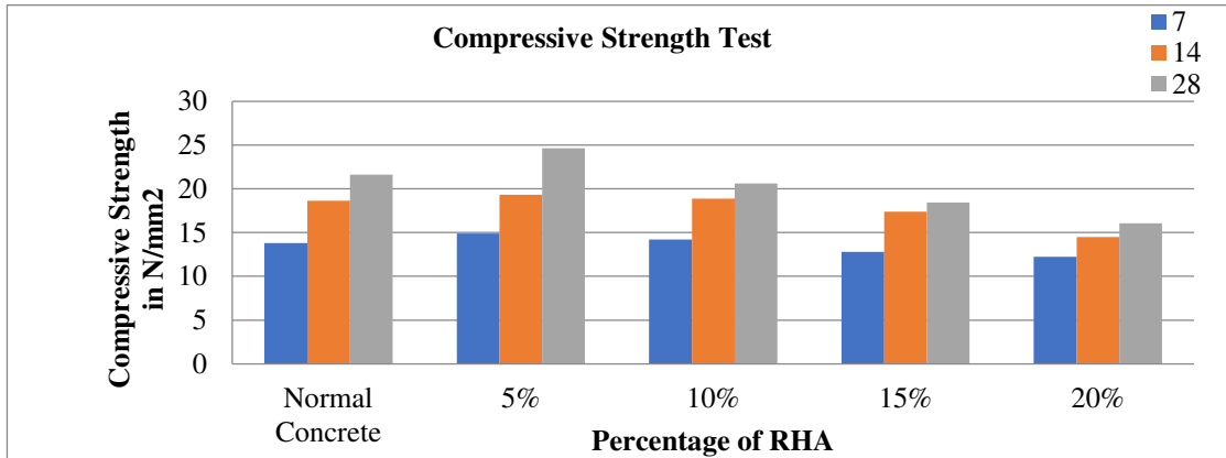
Figure 3: Compressive strength of concrete for varying percentage of RHA
