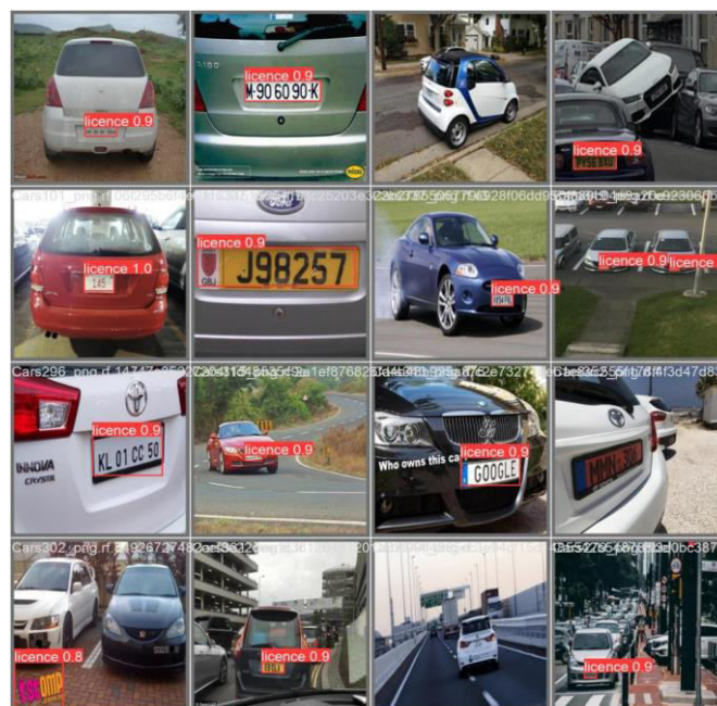
Fig :Licence plate recognition
