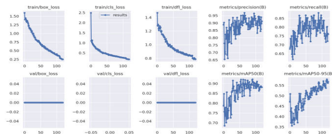
Fig:Metrix on object identification after testing the data
