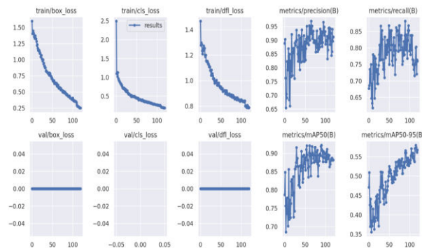
Fig: Metrix on object identification after testing the data
