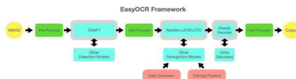
Fig:EasyOCR Framework
