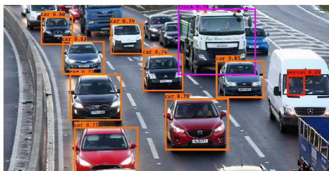
Fig:Vechile Recognition
