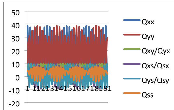
Graph (3.1): effect of changed lamina orientation on stiffness properties
