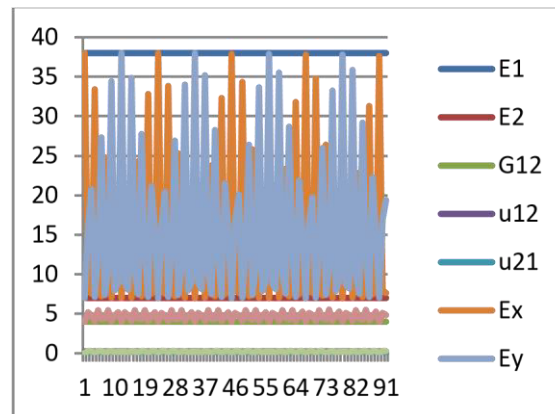
Graph (3.8): Effect of lamina changed orientation on off-axis and on-axis engineering elastic constants.
