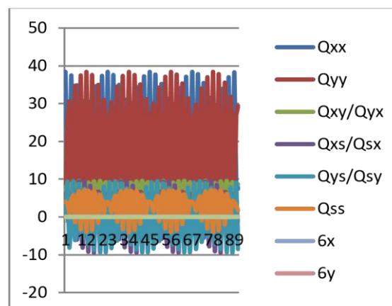
Graph (3.4): Effect of laminas stiffness components on off-axis stress
