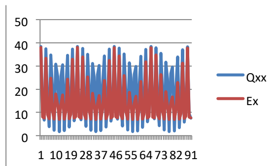
Graph (3.2): Effect of change of stiffness with respect to orientation on laminas engineering elastic properties
