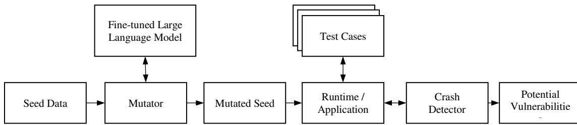
Figure 3 Generative AI based system design for vulnerability research
