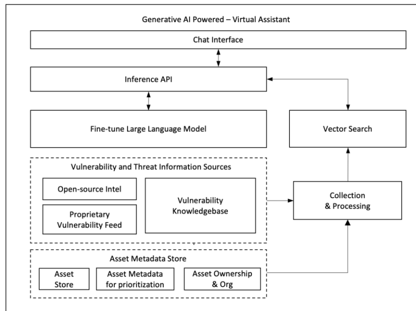
Figure 4 Generative AI-based system design for vulnerability remediation
