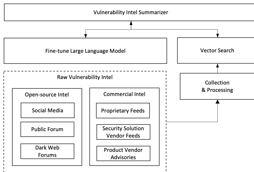
Figure 2 System design AI-based vulnerability intelligence system
